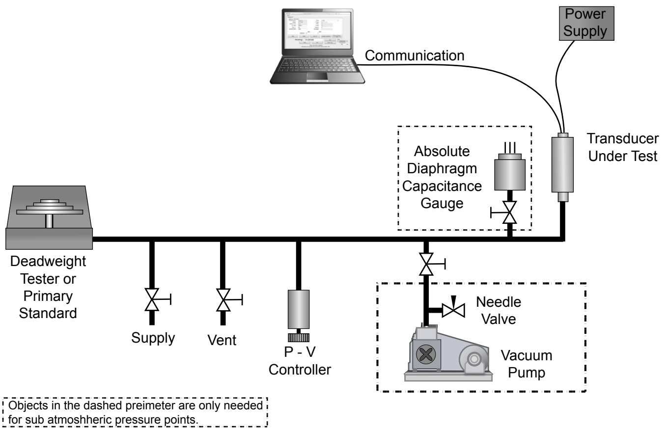
Figure 7.2.5 - Calibration Setup
