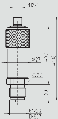
com M12 x 1 conector circular
