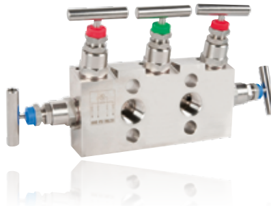
Valve manifolds for shutting off, pressure compensating as well as purging and venting differential pressure measuring instruments
