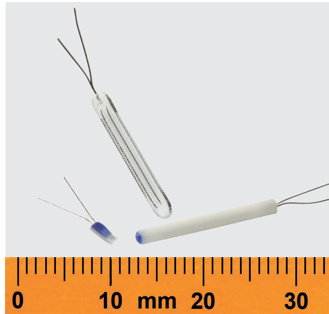
Fig. left: Thin-film measuring resistor
